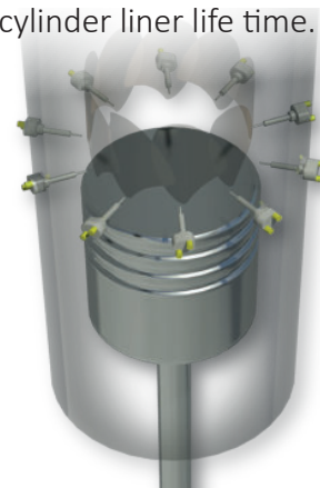
The HJ SIP use a swirl injection priciple that creates an optimal and uniform oil film on the cylinder wall.
